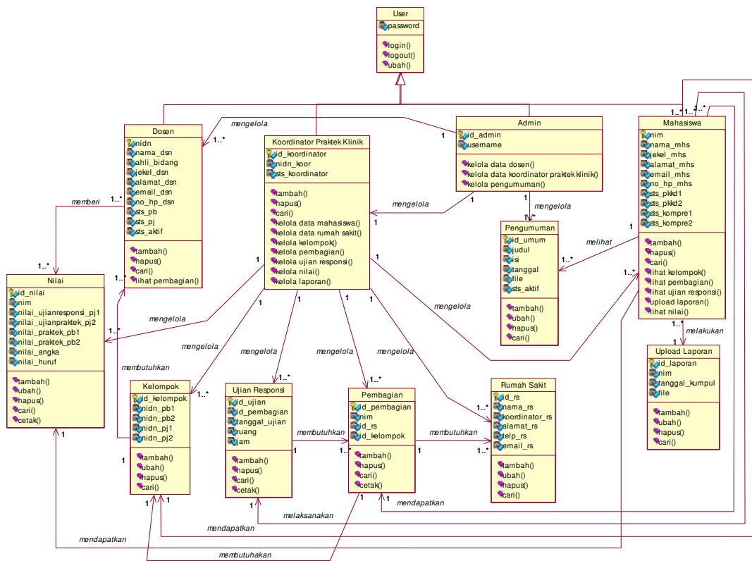
Gambar 2. Diagram Class
