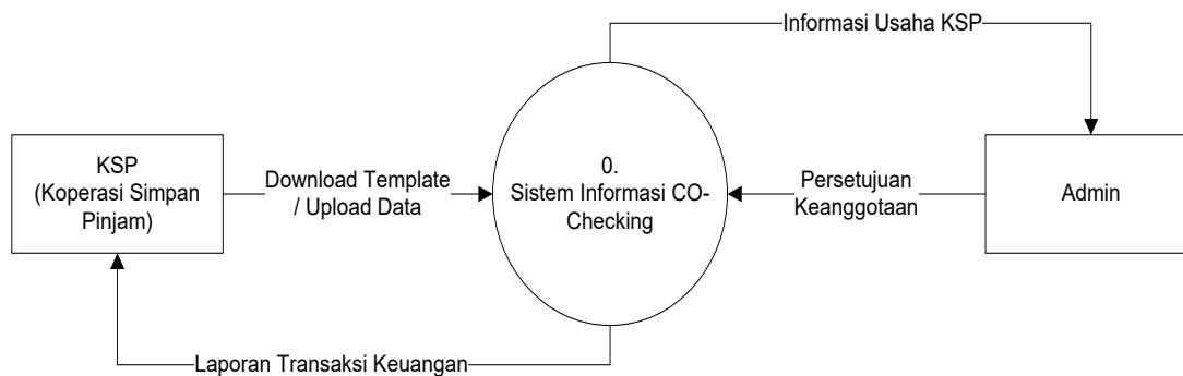
Gambar 3. Diagram Context
