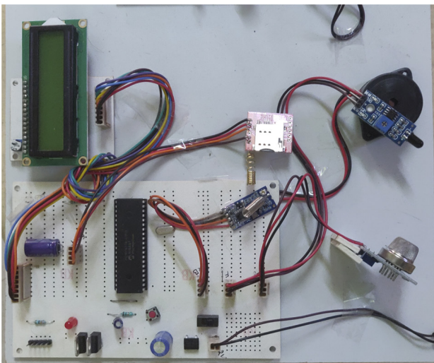
Figure 5: Master node of fire alert system with sensors and GSM modem.
