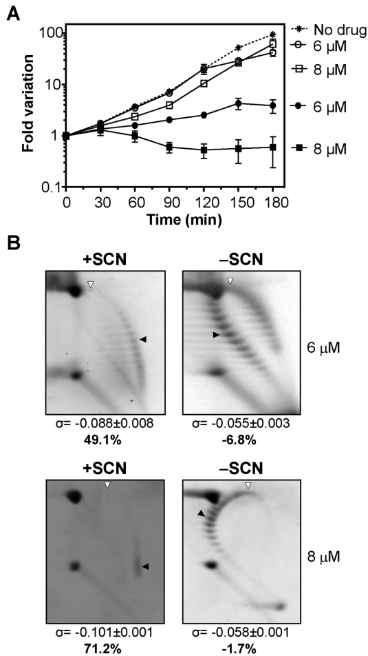
Figure 2. The removal of SCN led to a recovery in the cell viability and in the supercoiling density. (A) Viability of R6 (pLS1) cultures. Cultures were grown at an \text{OD}_{620\text{nm}} of 0.4 and diluted 100-fold in medium containing either 6 or 8 \mu\text{M} of SCN. After 120 min growth in the presence of the indicated amounts of SCN, cells were centrifuged, washed, and suspended in either drug-free medium (empty symbols) or in medium containing the same SCN concentrations (6 or 8 \mu\text{M} SCN, full symbols) than in the previous treatment. As control, a culture was grown at \text{OD}_{620\text{nm}} of 0.4, diluted 100-fold in drug-free medium and grown during 180 min (no drug). Samples were taken at the indicated times and plated in drug-free agar medium. Results are the average of three independent replicates \pm SEM. (B) Distribution of pLS1 topoisomers in 2D-agarose gel electrophoresis. Electrophoresis conditions and symbols are as indicated in the legend of Figure 1. Samples were taken after 120 min treatment with SCN (+SCN) and 120 min after removal of the drug (-SCN). Results are the average of at least three independent replicates \pm SD.
