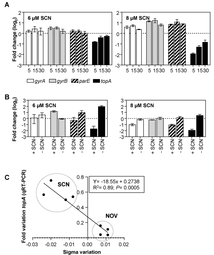
Figure 3. Changes in supercoiling levels affect the transcription of topA as measured by qRT-PCR. (A) Cultures of the R6 strain at an \text{OD}_{620\text{nm}} of 0.4 were treated with 6 or 8 \mu\text{M} of SCN. (B) Cultures were grown at an \text{OD}_{620\text{nm}} of 0.4 and diluted 100-fold in medium containing either 6 \mu\text{M} or 8 \mu\text{M} of SCN (+SCN) or in medium alone (-SCN). (C) Correlation between fold changes in supercoiling levels and changes in the transcription of topA . The data corresponds to samples treated with either SCN or NOV at concentrations that allowed cellular growth and recovery of DNA supercoiling: 4 and 6 \mu\text{M} ( 0.25 \times \text{MIC} and 0.375 \times \text{MIC} ) for SCN; 0.5 and 1 \mu\text{g/ml} ( 0.5 \times \text{MIC} , and 1 \times \text{MIC} ) for NOV. In both cases, time points of 15 and 30 minutes were used. The conditions of the qRT-PCR experiments and the normalization of the data are described in the Materials and Methods. In (A) and (B), values from three independent replicates (mean \pm SEM, n = 3 ) were normalized against values obtained at time 0 min.
