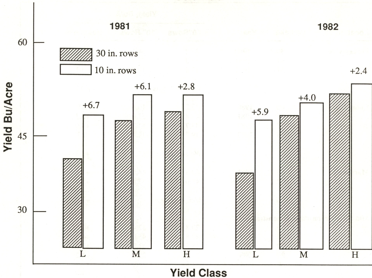
Figure 1. Yields of low (L), medium (M) and high (H) yielding groups of soybean varieties. Groupings are based on yields in 30-inch rows. In each case, the value at the top of the yield bar for 10-inch rows gives the response for drilling. Note that the greatest increases are for the group of varieties that produced the lowest yields. Yields from low-yielding varieties, despite the above-average increases, were not as good as those produced by the other groups. It is better, therefore, to select a variety based on its yield potential rather than the amount it responds to row spacing.
