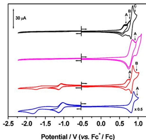
Figure 1. Cyclic voltammetry of P5A (black trace), [P5A-Rot] 2+ (magenta trace), P4A1Q (red trace) and P3A2Q (blue trace), in CH 2 Cl 2 containing [nBu 4 N][BF 4 ] (0.4 M) as supporting electrolyte, at ambient temperature and at 0.10 Vs -1 . Letters indicate potentials applied in bulk electrolysis and spectroelectrochemical experiments; first oxidation (A), second oxidation (B) and third oxidation (C).
