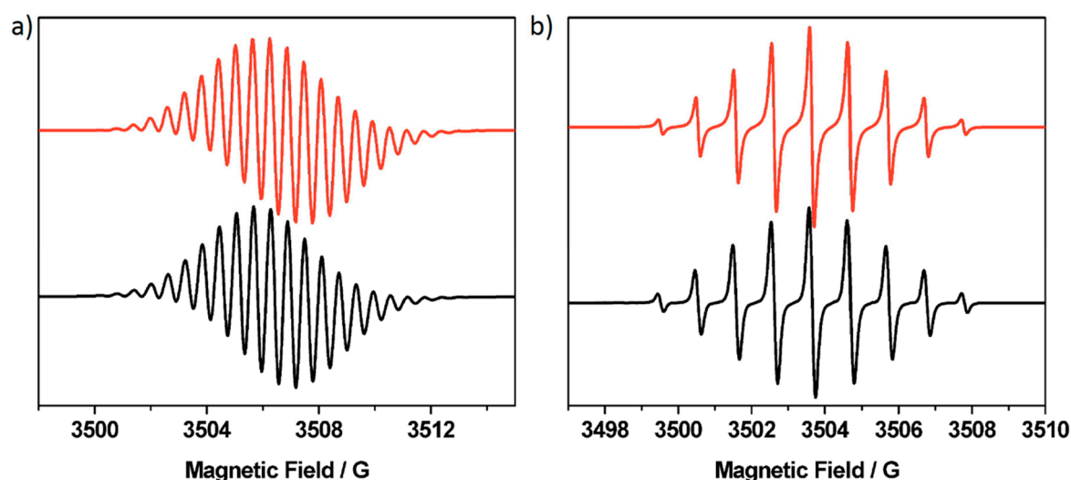
Figure 3. Experimental (black) and simulated (red) X-band EPR spectra of: (a) [P5A] + and (b) [P4A1Q] - . Samples were electrogenerated from the parent molecules at 273 K as CH 2 Cl 2 solutions containing [nBu 4 N][BF 4 ] (0.4 M) as the supporting electrolyte. Spectra were recorded at ambient temperature. Simulated spectra were generated using the parameters listed in Table 3.
