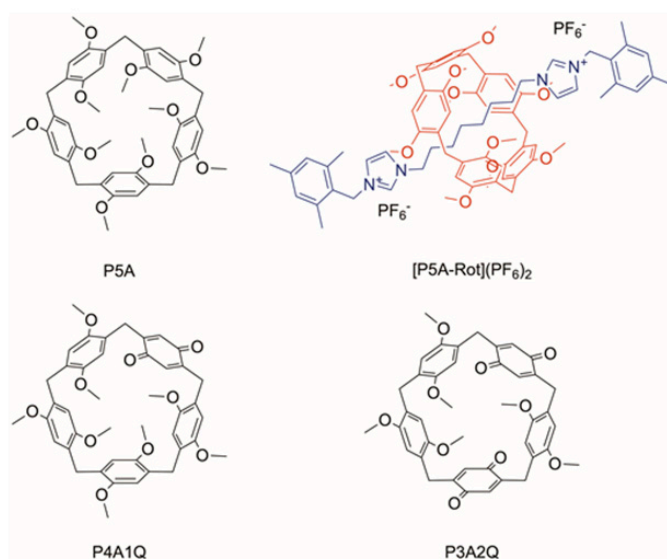
Scheme 1. Molecules investigated in this study.
