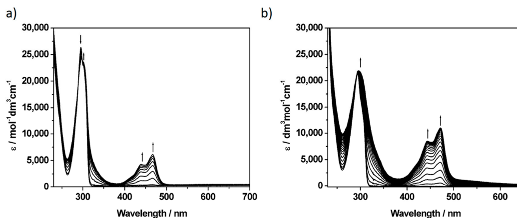
Figure 2. UV-vis absorption spectra showing (a) the inter-conversion of redox states in P5A between P5A and [P5A] + (potential A) (b) the inter-conversion of redox states in [P5A-Rot] 2+ upon oxidation at potential A. See Figure 1 for potentials applied. Spectra were recorded in CH 2 Cl 2 containing [nBu 4 N][BF 4 ] (0.4 M) as the supporting electrolyte at 273 K.
