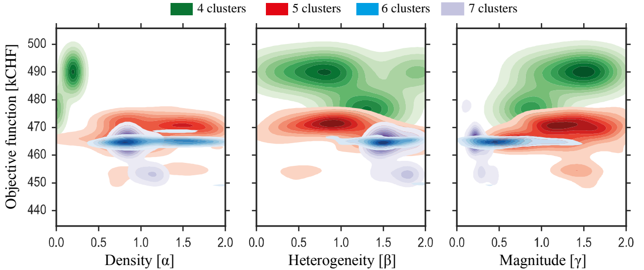
Fig. 6. Density estimation of the fitness value after optimisation based on the weights of the combined clustering algorithm: density (a), heterogeneity index (b) and loads magnitude ( \gamma ).
