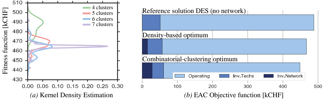
Fig. 5. Difference in the optimal solution for different weights of the clustering score function: (a) Fitness function kernel density estimation. (b) Equivalent annual cost (EAC) for the reference case, density-based case and combined clustering case.
