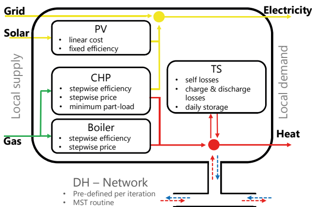
Fig. 1. Energy hub design space
