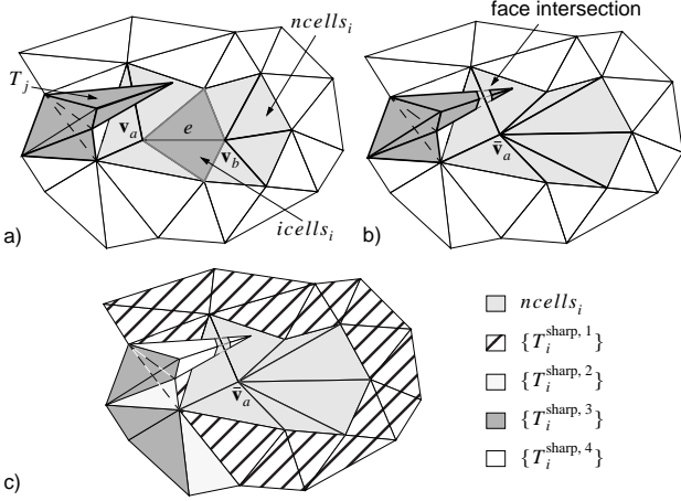
Figure 4: Tetrahedron T_j intersects two faces of \{f_k\} after collapsing edge e_i into vertex \bar{\mathbf{v}}_a . a) before collapse. b) after collapse. c) Traversal of the mesh \{T_i^{\text{sharp}, m}\} for iteration steps 1–4.
