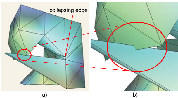
Figure 1: Intersection of two tetrahedra: a) The edges of two non-adjacent tetrahedra bounding the volume intersect while collapsing an edge in a locally concave mesh region. b) Close-up of the intersection.
