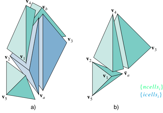
Figure 2: Edge collapse in a tetrahedral mesh: a) Mesh before collapsing edge (\mathbf{v}_a, \mathbf{v}_b) . b) Configuration after collapse with resulting vertex \bar{\mathbf{v}}_a . (Tetrahedra are shrunk to emphasize the underlying 3-dimensional structure.)
