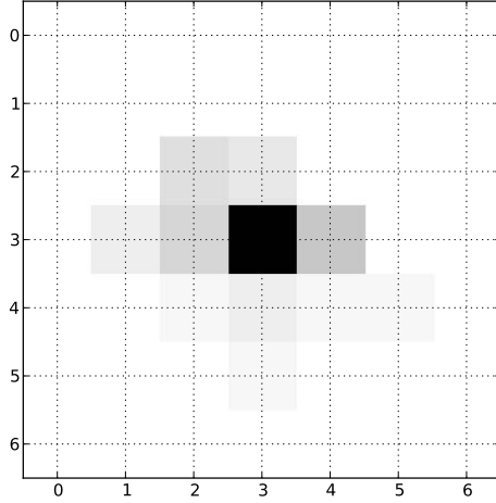
Figure 5. P(IP\_local_{t+1}|IP\_local_t = (3, 3))
