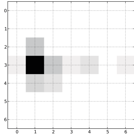
Figure 4. P(IP\_local_{t+1} | IP\_local_t = (3, 1))
