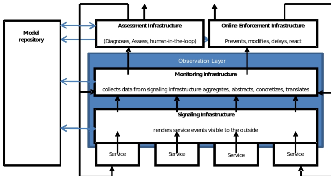
Figure 1.1: MASTER components, [19]
