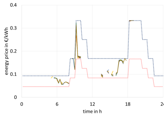
Figure 7. Energy prices of selling prosumers for the system without BES units: a) centralized model, b) last iteration of the ADMM procedure.
