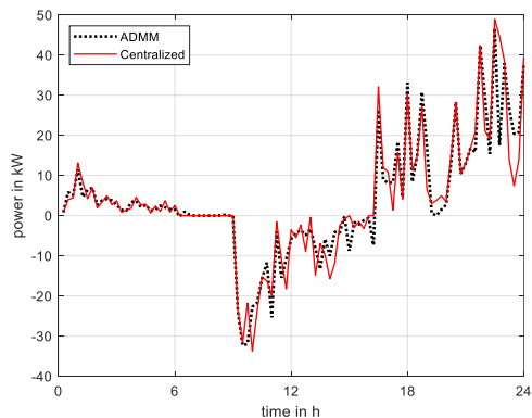
Figure 5. Comparison of the profiles of the power exchanged with the utility grid obtained by using the centralized and the distributed approach: a) without BES units and b) with BES units. Positive values indicate imported power from the utility grid, negative values indicate exported power to the utility grid.
