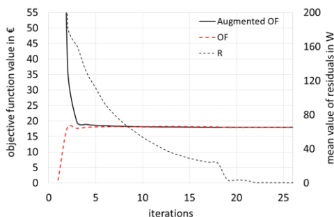
Figure 4. ADMM convergence (augmented OF , part of OF corresponding to the power exchanged with the utility grid, average of primal residuals at each iteration): a) without BES units, b) with BES units.
