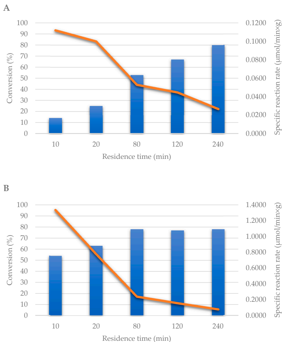
Figure 1. Screening of the residence time for the synthesis of ara-A (vidarabine, 11 ). (A) enzymes immobilized on glyoxyl-agarose; (B) enzymes immobilized on EziG™1. Experimental conditions: [araU] = 16 mM; [Ade] = 8 mM; 50 mM phosphate buffer pH 7.5; T = 28 °C; P = 20 psi. Conversions (%; blue bars) were determined by HPLC (see Materials and Methods for details). Specific reaction rates ( \mu\text{mol min}^{-1} \text{g}^{-1} ; orange line) were calculated using the equation: r = [P] \times f/m_e , where [P] is the concentration of the product ( \mu\text{mol mL}^{-1} ), f is the flow rate ( \text{mL min}^{-1} ) and m_e is the amount of immobilized enzyme (g) [23].
