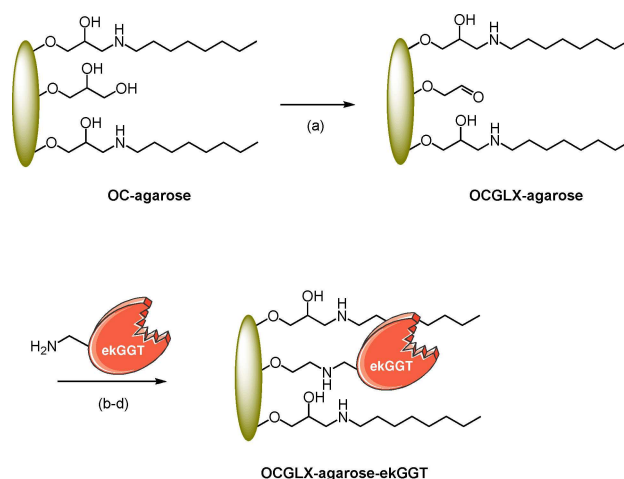
Scheme 1. Immobilization of ekGGT on OCGLX-agarose. Experimental conditions: (a) 35 \mu\text{mol NaIO}_4 per g carrier, r.t., 2 h; (b) ekGGT ( 1 \text{ mg g}^{-1} ), \text{KH}_2\text{PO}_4 (pH 7, 0.025 M), r.t., 3 h; (c) OCGLX-agarose-ekGGT, \text{NaHCO}_3 (pH 10, 0.05 M), r.t., 3 h; (d) \text{NaBH}_4 , pH 10, 30 min.
