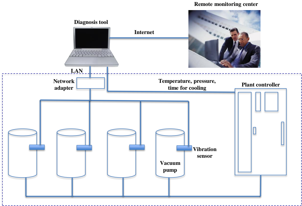
Figure 11: Prototype of the diagnosis system
