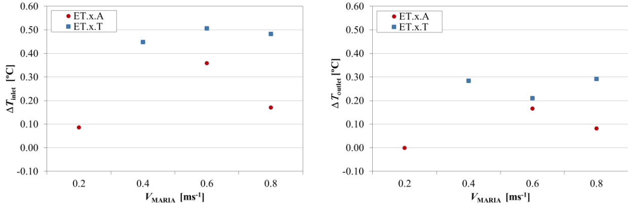
(a) Variation of inlet air temperature.
