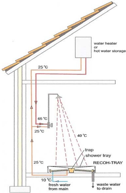
Fig. 1. Home shower heat exchanger (HX) system.
