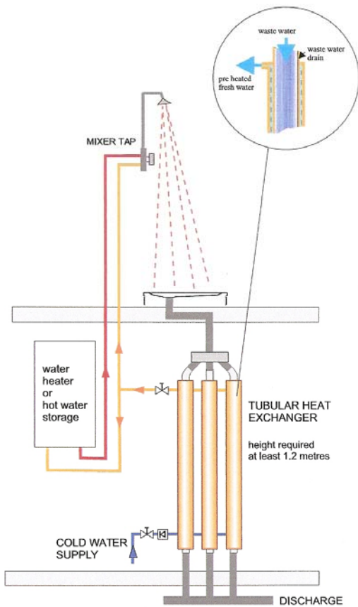
Fig. 2. Swimming pool shower heat exchanger (HX) system.
