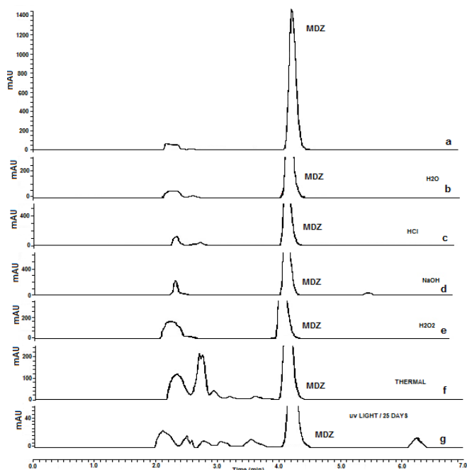
Figure 1. Chromatograms obtained under stress studies. a) MDZ IPA solution (150 \mu\text{g}\cdot\text{mL}^{-1} ); b) After neutral hydrolysis; c) After acid hydrolysis; d) After alkaline hydrolysis; e) After oxidative degradation; f) After thermal degradation; g) After 25 days of exposure in UV light. Chromatographic conditions: \text{C}_{18} column, mobile phase consisting of methanol: acetonitrile: water (45:35:20 v/v/v) with 0.4% triethylamine pH 6.5 under flow rate of 1.0 \text{mL}\cdot\text{min}^{-1} and UV detection at 235 nm.
