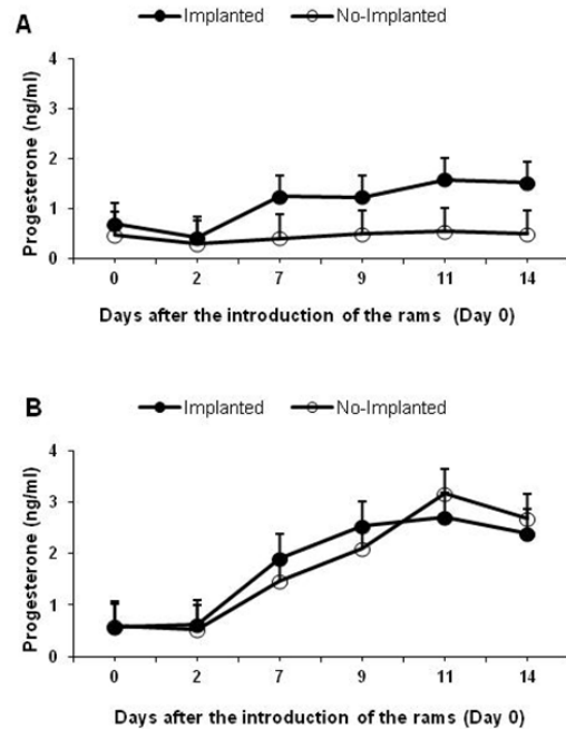
Figure 2. Plasma progesterone concentrations (mean ± S.E.M.) in implanted and no-implanted Romney Marsh (A) and Suffolk (B) ewes determined at the same day of the introduction of the rams (Day 0) and 46 days after melatonin implantation. P > 0.05 .
