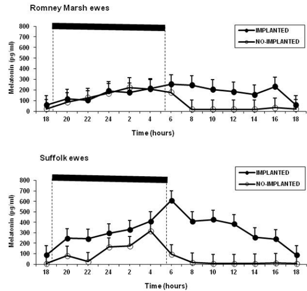
Figure 1. Plasma melatonin concentrations (mean ± S.E.M.) in implanted and no-implanted Romney Marsh and Suffolk ewes determined at 2-hs intervals during a 24-hs period at 43 days after melatonin implantation. The dark-phase of the day is indicated in upper panel. * P < 0.01.
