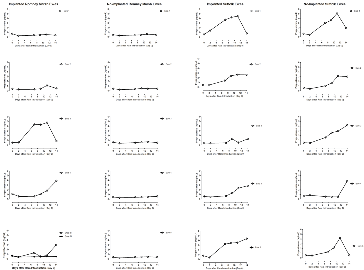
Figure 4. Individual plasma progesterone concentrations in melatonin implanted and no-implanted Suffolk ewes determined at the same day of the introduction of the rams (Day 0) and 46 days after melatonin implantation.
