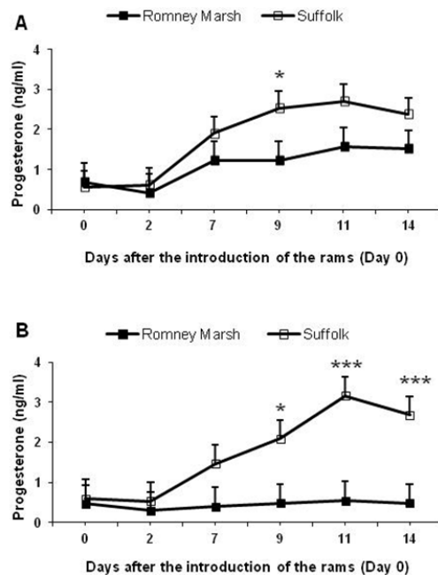
Figure 3. Plasma progesterone concentrations (mean ± S.E.M.) in implanted (B) and no-implanted (A) Romney Marsh and Suffolk ewes determined at the same day of the introduction of the rams (Day 0) and 46 days after melatonin implantation. * P < 0.05 ; *** P < 0.001 .
