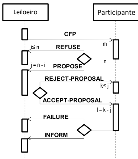
Figura 1. Protocolo Contract-Net [13]
