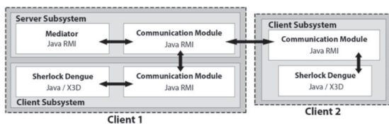
FIGURE 4 – SDv6 communication architecture. SOURCE: Our authorship
