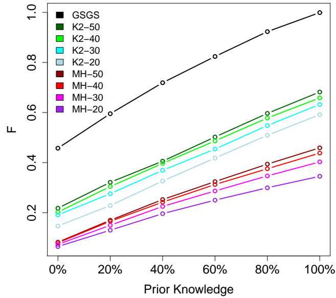
Figure 5.4: Network: E. coli . Comparison of the GSGS approach with K2 and MH in terms of F-Scores. Upper Panel: Using discrete measurements; Lower Panel: Using continuous measurements with different sample sizes.
