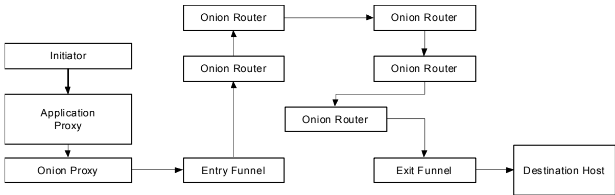
Figure 3: Onion Routing
