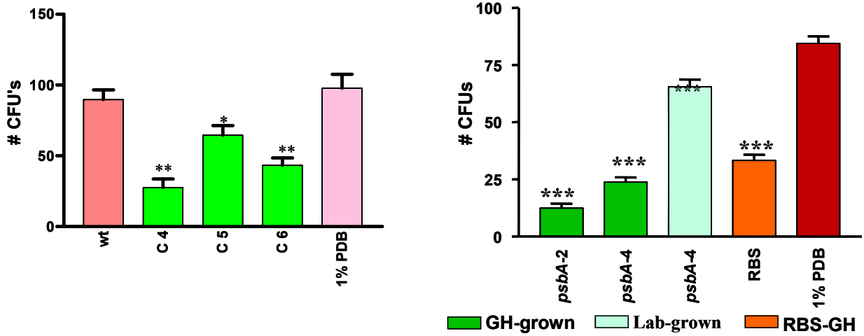
A. Performance of RBS plants. B. Performance of psbA 5'UTR plants as affected by light intensity. On this graph psbA -2 & 4 correspond to pC2 & pC4; RBS corresponds to C4. Asterisks (*, **, ***) are indicative of confidence levels, 95%, 99%, and 99.9% respectively; n=3. Abbreviation: colony forming unit (CFU).
