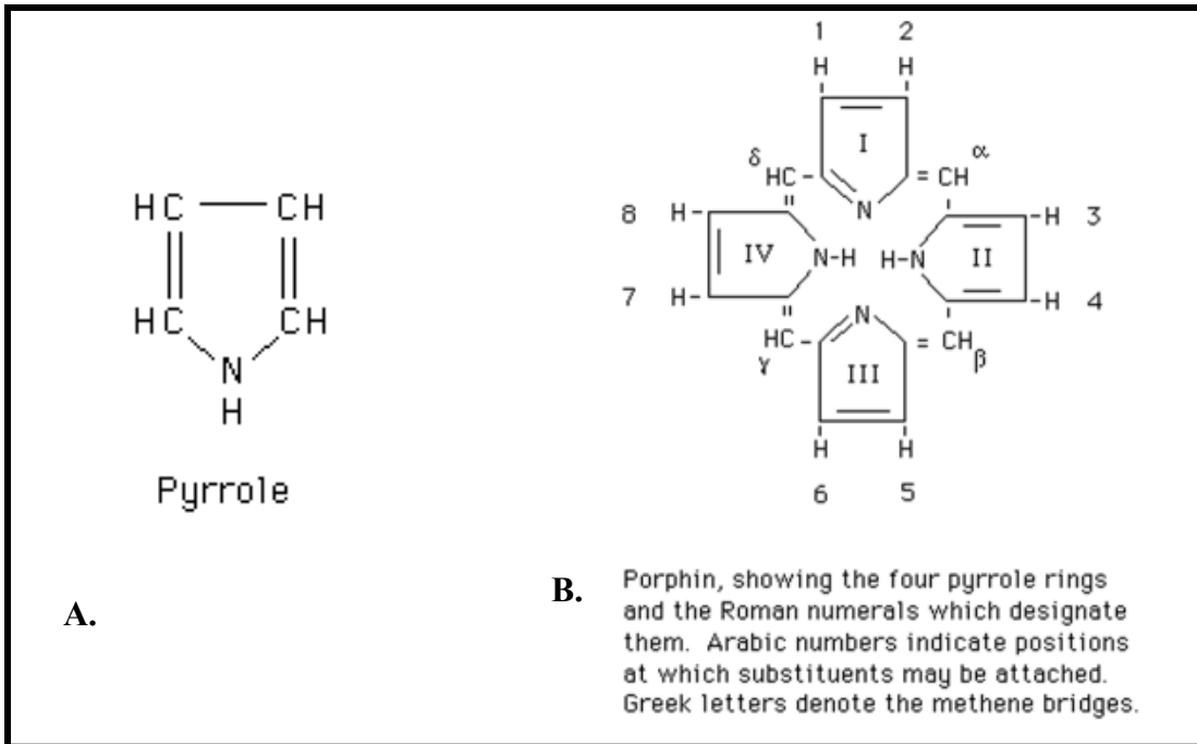
Figure 4-4: Representation of pyrrole and porphin. A) Pyrrole molecule. B) Structure of porphin, a tetrapyrrole.
