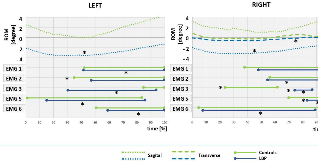
Figure 51. Phase 2 EMG onsets/offsets and ROM. Only first EMG onsets/offsets displayed. EMG activation when significant between groups is indicated with a * under the respective EMG onset line ( p < .05 ). Significant difference in onset time between groups is indicated with a * to the left of the respective EMG onset line ( p < .05 ). Significant difference between groups in ROM is indicated with a * at the respective plane of motion ( p < .05 ).
