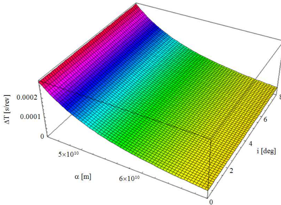
Fig. 2. The anomalistic period time change of Mercury due to Lense-Thirring effect as a function of a and i by supposing that their values are altered in the ranges [\text{perihelion-aphelion}] and [0, 8] , respectively
