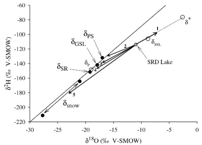
FIGURE 3. Potential isotopic trajectories of a theoretical Slave River Delta (SRD) lake in response to (1) evaporation, (2) thaw season precipitation ( \delta_{\text{PS}} ; Gibson and Edwards, 2002), (3) Great Slave Lake ( \delta_{\text{GSL}} ) exchange, (4) Slave River ( \delta_{\text{SR}} ) flooding, and (5) snowmelt ( \delta_{\text{snow}} ) input, superimposed on the 2003 isotopic framework (see Fig. 2). Isotopic framework parameters are shown as open circles. In this example, the theoretical lake is shown to plot on the Local Evaporation Line (LEL), indicating the lake is fed by water of isotopic composition similar to mean annual precipitation.
