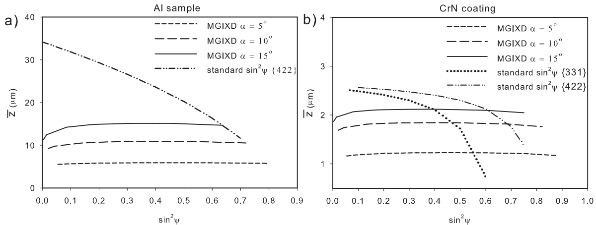
Fig. 2. Information depth \bar{z} vs. \sin^2 \psi calculated from Eq. (4) for Al (a) and CrN (b) materials using Cu radiation. Results for the MGIXD (different \alpha angles) and for the standard \sin^2 \psi methods ( \Omega mode) are shown. In the case of CrN the calculations correspond to the coating thickness equal to t = 6 \mu\text{m} , while an infinite sample thickness was assumed for aluminium.
