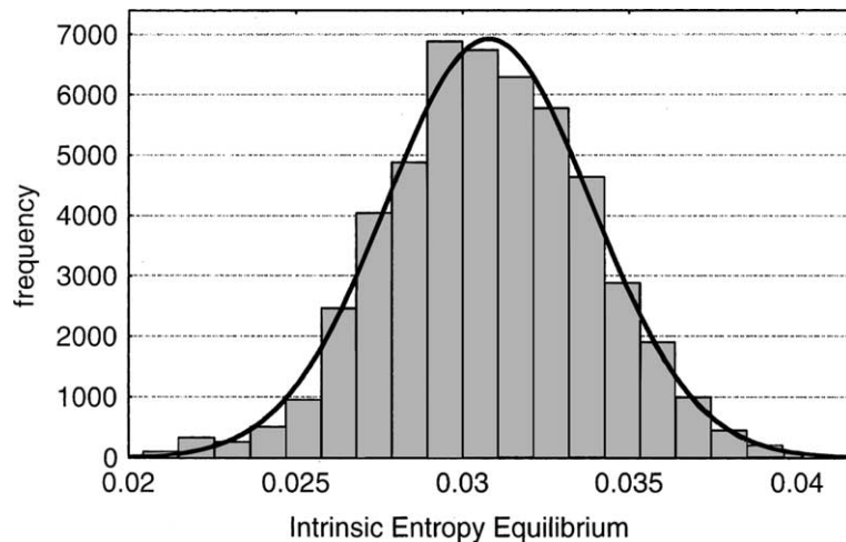
Fig. 3. Histogram of intrinsic entropy S_0^{Eq} at equilibrium for a system size of 32^2 cells. The histogram is obtained by 50,000 simulations of the equilibrium and the Gaussian PDF is plotted with mean \mu_{S_0^{Eq}} = 0.0308 and standard deviation of \sigma_{S_0^{Eq}} = 0.00308 .
