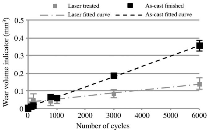
Fig. 5. Wear test results.
