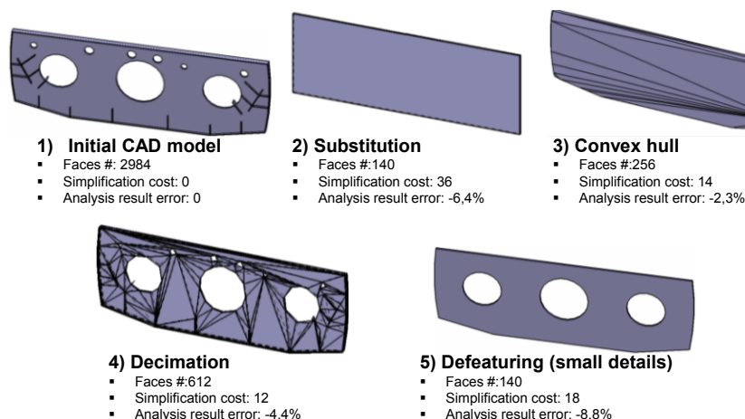
Fig. 4: Examples of CAD model simplification
