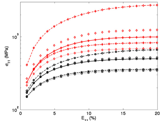
Fig. 11. Evolution of the model predictions when: the layer thickness \lambda is divided by a factor of 10 with respect to its value in Table 2, i.e. \lambda = 0.03 \mu\text{m} (dashed lines), k_{gnd}=0 (dotted lines), an aspect ratio of 2 is accounted for in the tensile direction (mixed lines), an aspect ratio of 1.5 is considered normal to the tensile direction (full lines), and, particles are assumed spherical (no lines). The circles and diamonds denote the macroscopic stress and the stress in cementite particles, respectively.
