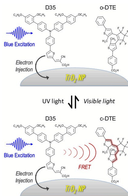
Fig. 1 Photophysical pathways for the excited D35 dye sensitizer when the DTE dye is switched between its ring-open (o-DTE) and ring-closed (c-DTE) isomers. When c-DTE is present it acts as a FRET acceptor, reducing the efficiency of the D35 dye's electron injection into the conduction band of the titania nanoparticle.
