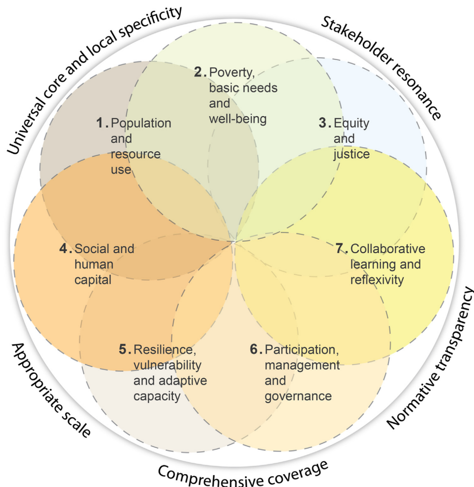
Fig. 3. Social-ecological dynamics of coastal ecosystems: a conceptual framework.
