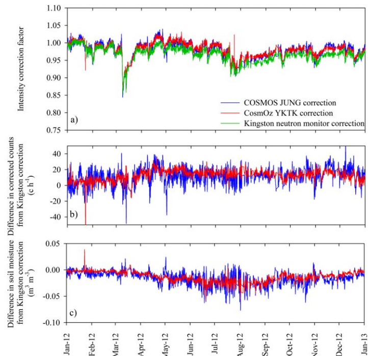
Figure 6. (a) Cosmic-ray neutron intensity correction factors at Tullochgorum using local Kingston neutron monitor (baseline case) and comparison with correction factors using CosmOz approach (nearest cutoff rigidity neutron monitor from NMDB.eu; i.e., Yakutsk, YKTK) and COSMOS approach using neutron monitor measurements from Jungfrauoch (JUNG) scaled by rigidity cutoff. Difference in corrected counts (b) and soil moisture estimate (c) at Tullochgorum using CosmOz and COSMOS approaches when compared to the corrected counts using the Kingston neutron monitor.
