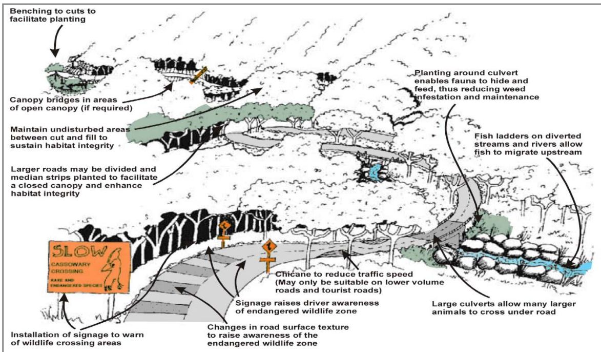
(Top) Faunal movement is inhibited by embankments (shown in the graphic on the left) and enhanced by bridges (shown on the right). (Bottom) Designing for safe faunal movement across roads can be done using multiple approaches.
