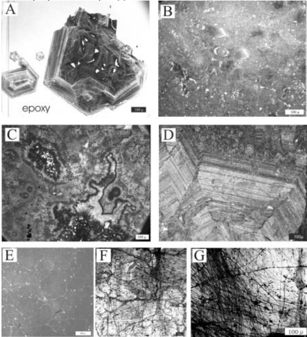
Figure 2. All images are SEM-CL images and show only vein quartz, except where noted. All scale bars are 100 microns. A) Euhedral growth zones in experimentally grown quartz. Bright spots within the large crystal are holes. B) Bi-pyramidal euhedral quartz from the massive sulfide deposit from West Shasta, CA. C) Complex chalcidonic and spheroidal textures in quartz from the McLaughlin epithermal deposit CA. D) Euhedral growth zones in vein quartz from an epithermal Main Stage vein in Butte, MT. E) Homogenous CL-dark quartz from the San Bento orogenic gold deposit in Minas Gerais, Brazil F) Splatter and cobweb
