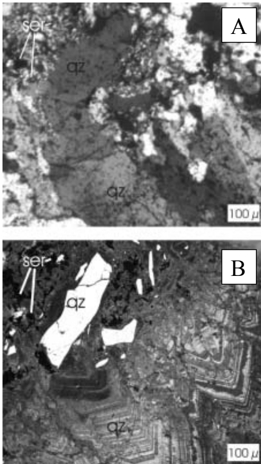
Figure 1. A) Transmitted light image of a pyrite-quartz vein. Image shows that both quartz and sericite are present in the vein, but little more. B) SEM-CL image of the same area shown in A. This image shows a variety of CL textures including evidence for multiple generations of quartz growth.
