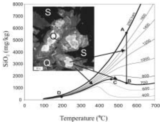
Figure 3. Solubility of quartz in water as a function of temperature at pressures indicated (data from Shock et al., [11]). Path A-B represents an isothermal pressure drop from lithostatic (2000 bars) to near hydrostatic pressure (700 bars) at 550°C causing quartz precipitation. Cooling along path B-C at 700 bars (in the zone of retrograde quartz solubility) leads to dissolution of quartz. Cooling below point C at 700 bars causes quartz to precipitate. Such a depressurization/cooling path is
