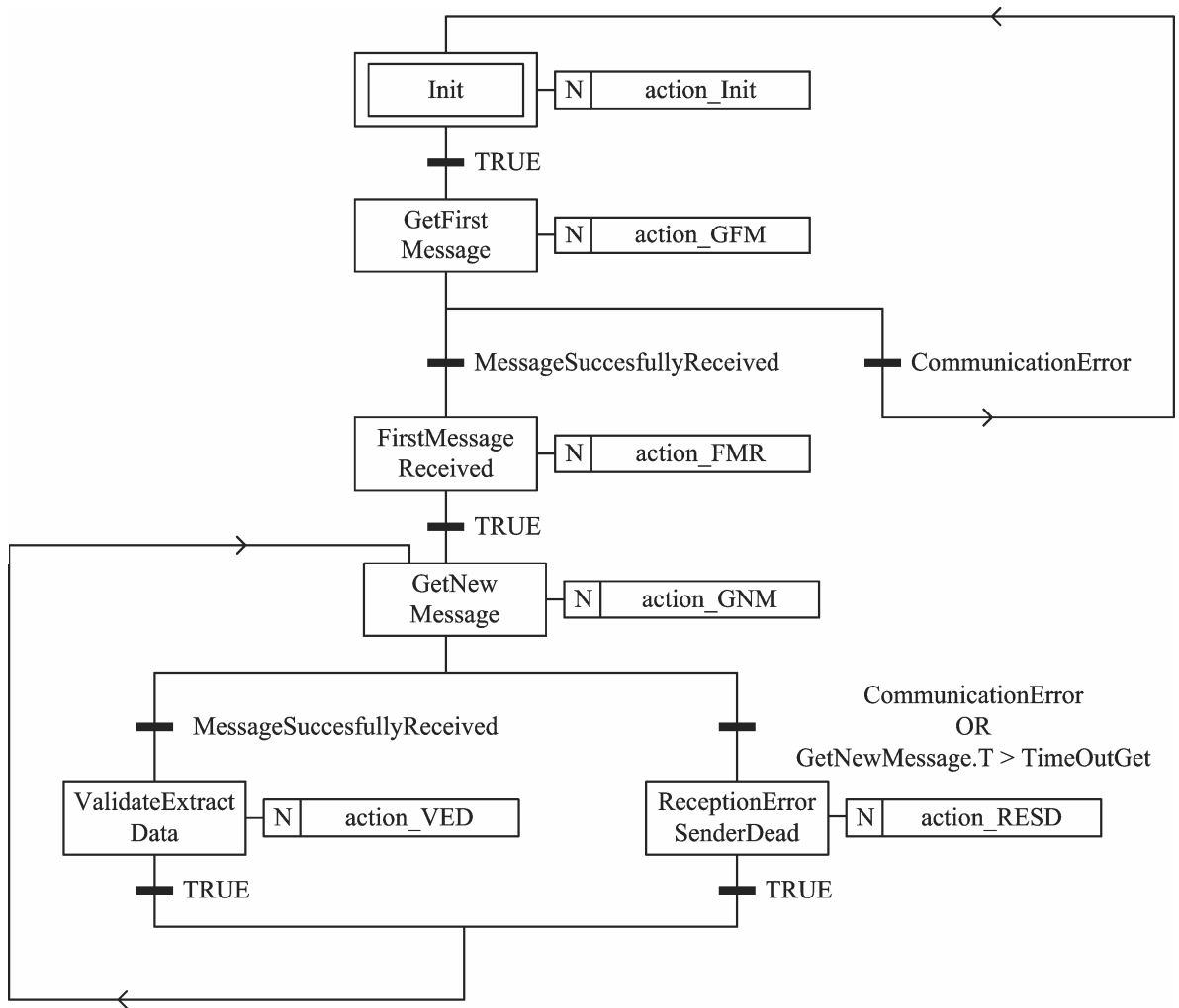
Figura 6.4 – SFC Receiver
