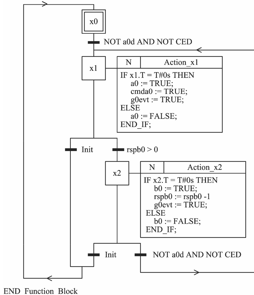
Figura 4.2 – Function Block g0
