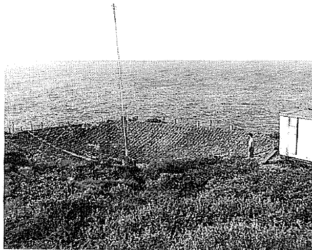
Figure 2. The 21.9m antenna in June 1952, with the small instrument hut on the extreme right. (ATNF Historic Photographic Archive:2763-3)
