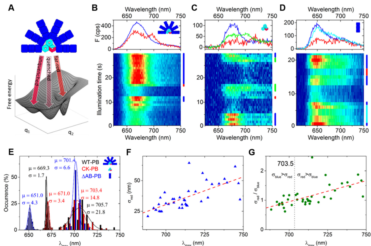
Fig. 3. (A) By means of reversible switches between different conformational states, illuminated PBs assume different minima in their free energy landscape, portrayed here as a function of two nuclear coordinates, which are signified by three major spectroscopic states: unquenched, quenched and far-red. Room-temperature F spectral sequence of a single WT-PB (B), CK-PB (C), and \Delta AB-PB (D). Spectra on top are averages of the spectra in the map corresponding to the times indicated by the color-coded bars on the right of each spectral trace. In (E), peak distributions of far-red emission bands ( \lambda_{\max} > 680 nm, 5-nm bins) compared to peak distributions of ensemble-like spectra (i.e., devoid of far-red emission bands) ( \lambda_{\max} < 680 nm, 1-nm bins). Each distribution is scaled separately. The total number of quasi-stable, reversible, far-red spectra are 46, 67, and 83 from 42 WT-PB, 42 CK-PB and 44 \Delta AB-PB complexes, respectively, selected from a few hundred individually measured complexes (the selection allows to focus on intact, biologically relevant complexes only). Fitting details are described in the Experimental section and an example is shown in Fig. S5. For spectra devoid of far-red emission bands, only unquenched states were considered to enhance the fitting accuracy. Since \lambda_{\max} of \Delta AB-PB's 672-nm band was fixed it is not shown. Gaussian fits of the peak distributions are displayed (black curves), along with the mean value ( \mu , in nm) and the full-width at half-maximum ( \sigma , in nm) of each fit. In (F), relationship between the full-width at half-maximum and peak position of the far-red emission bands from WT-PB. In (G), ratio of the full-width at half-maximum of the far-red and blue bands of spectra with far-red emission as a function of the far-red spectral peak. The dashed lines in (F and G) denote linear regressions. Dotted vertical line in (G) is at 703.5 nm. In (B, C, D and E), the right insets denote the types of PB complexes used for the measurements. (For interpretation of the references to color in this figure legend, the reader is referred to the online version of this chapter.)
