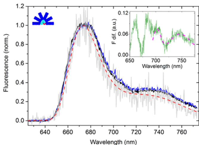
Fig. 2. Room-temperature bulk spectrum of WT-PB (black) compared with the average of 4000 randomly selected single molecule spectra (blue) and a representative 10-s averaged single molecule spectrum of a WT-PB complex in an unquenched state (gray). For bulk, a 12 nM solution of freely diffusing complexes was excited; each single molecule spectrum originated from a different substrate-bound WT-PB complex. Spectra were measured consecutively on the same optical setup. A 4-min averaged background spectrum was subtracted from the black and blue spectra and a 10-s averaged background spectrum was subtracted from the gray spectrum. The right inset shows the difference between the bulk spectrum (black) and the double skewed Gaussian fit (red dashed line) of the single-molecule spectrum. The red part of the difference spectrum was fitted with two Gaussians (magenta dashed line) with peak positions at 702 and 746 nm. The left inset denotes the type of sample used in the measurements (WT-PB).
