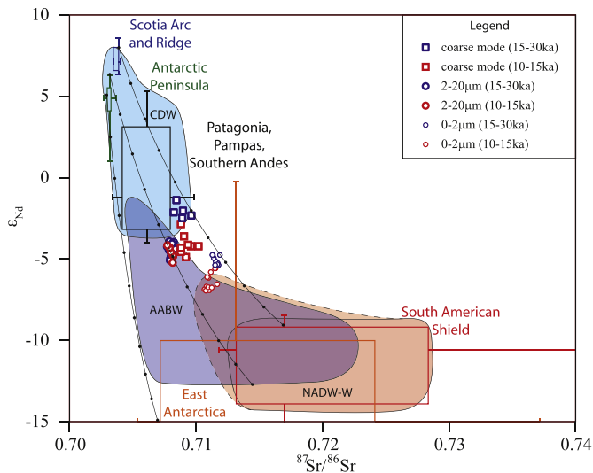
Fig. 6. ^{87}\text{Sr}/^{86}\text{Sr} - \epsilon_{\text{Nd}} diagram of MD07-3076Q sediments and of potential sources of sediments for the South Atlantic Basin. Boxes representing the reference data delimit the first and the third quartile. The median values are represented by horizontal and vertical lines attached to the boxes for the \epsilon_{\text{Nd}} and the ^{87}\text{Sr}/^{86}\text{Sr} ratios, respectively. The short strokes at the end of these lines represent the 10th and 90th percentile values. Accordingly, the box represent 50% of values found for each potential provenance, and 80% is represented with the lines. Data sources: South American Shield- Allègre et al. (1996); Basile et al. (1997); Walter et al. (2000); de Mahiques et al. (2008); Jeandel et al. (2007), and references therein; Mallmann et al. (2007); Ganade de Araujo et al. (2014); Fuck et al. (2014); -Patagonia, Pampas, Southern Andes- Stern et al. (1990); Grousset et al. (1992); Basile et al. (1997); Walter et al. (2000); Smith et al. (2003); Jeandel et al. (2007), and references therein; Khondoker et al. (2018); -Scotia Arc and Ridge- Jeandel et al. (2007); Harrison et al. (2003); -Antarctic Peninsula- Hole et al. (1993); Kosler et al. (2009); Roy et al. (2007); Lee et al. (2005); -East Antarctica- DePaolo et al. (1982); Luttinen et al. (1998, 2010); Roy et al. (2007); Will et al. (2010).
