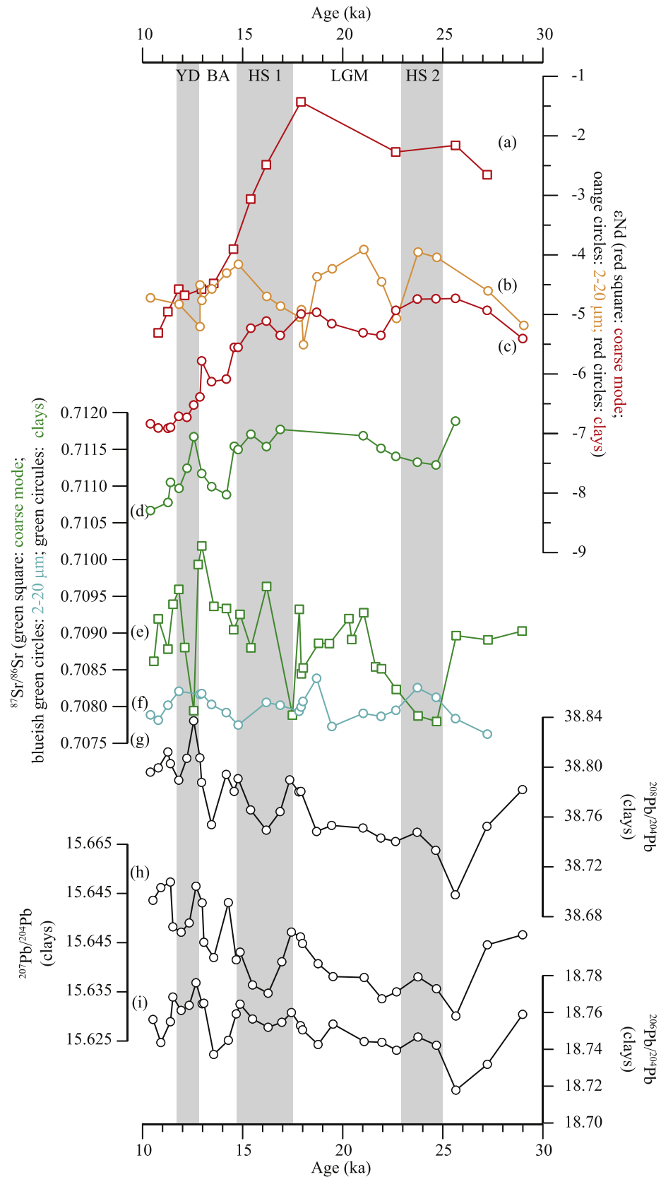
Fig. 5. Isotopic results from core MD07-3076Q. (a) \epsilon_{Nd} from the sortable silt mode fraction (20–32/40 \mu\text{m} ); (b) \epsilon_{Nd} from the cohesive silt mode fraction (2–20 \mu\text{m} ); (c) \epsilon_{Nd} from the clay-size fraction (<2 \mu\text{m} ); (d) ^{87}\text{Sr}/^{86}\text{Sr} from the clay-size fraction (<2 \mu\text{m} ); (e) ^{87}\text{Sr}/^{86}\text{Sr} from the sortable silt mode fraction (20–32/40 \mu\text{m} ); (f) ^{87}\text{Sr}/^{86}\text{Sr} from the cohesive silt mode fraction (2–20 \mu\text{m} ); (g) ^{87}\text{Sr}/^{86}\text{Sr} from the clay-size fraction (<2 \mu\text{m} ); (h) ^{208}\text{Pb}/^{204}\text{Pb} , (i) ^{207}\text{Pb}/^{204}\text{Pb} , and (j) ^{206}\text{Pb}/^{204}\text{Pb} from the clay-size fraction (<2 \mu\text{m} ).
