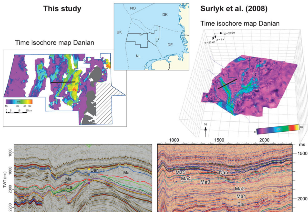
Figure 14. (Colour online) Comparison of the Danian channel found in this study (left) and the Danian channel identified by Surlyk, Jensen & Engkilde (2008) in the German Schill Grund High (right). Both study areas are indicated on the map. The time isochore maps of the Danian Ekofisk Formation show anomalies that are visible in the seismic sections below as deep Danian channels that cut into the top of the Maastrichtian. The black lines show the locations of the seismic sections, and the grey areas on the left map indicate the absence of the Chalk Group. The grey striped areas indicate where no reliable Danian thicknesses could be interpreted and the Danian is absent in the white areas. Abbreviations: Dan = Danian, Ma = Maastrichtian, Ca = Campanian.
