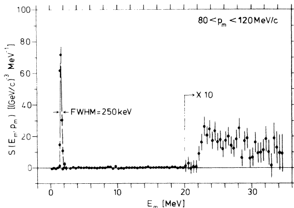
FIG. 1. Missing-energy spectrum of the {}^6\text{Li}(e, e'd) reaction.
