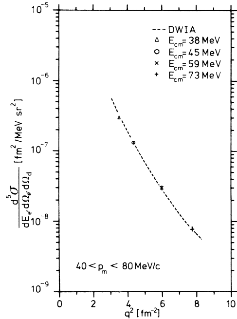
FIG. 4. Measured cross sections for the reaction {}^6\text{Li}(e,e'd){}^4\text{He}(\text{g.s.}) as a function of the momentum transfer squared. The dashed curve indicates the expected behavior (normalized at the highest q ) of the cross section for direct deuteron knockout, corrected for distortion effects.
