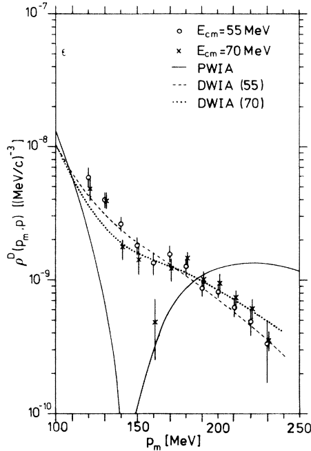
FIG. 3. Momentum distribution for the reaction {}^6\text{Li}(e,e'd){}^4\text{He}(\text{g.s.}) for 120 \leq p_m \leq 230 MeV/c, measured at two \alpha - d center-of-mass energies. DWIA curves are for the indicated center-of-mass energies. Each data point represents an average over a 10-MeV/c bin.
