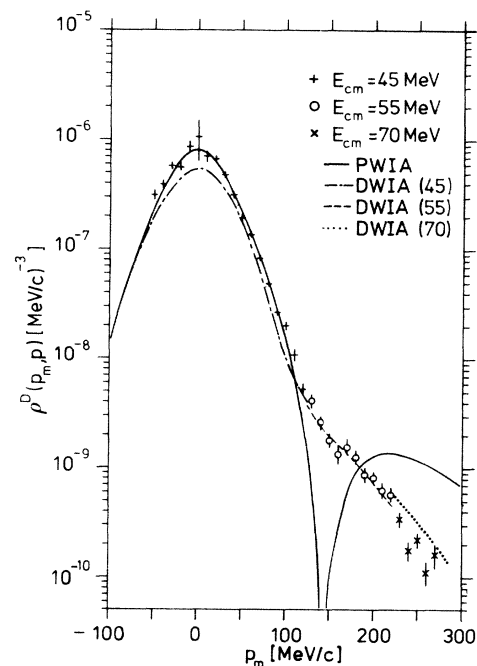
FIG. 2. Measured momentum distribution for the reaction {}^6\text{Li}(e, e'd){}^4\text{He}(g.s.) compared with the results of DWIA calculations, which use the "repulsive" wave function of Ref. 11. DWIA curves are for the indicated center-of-mass energies. Each datum point represents an average over a 10-MeV/c bin.
