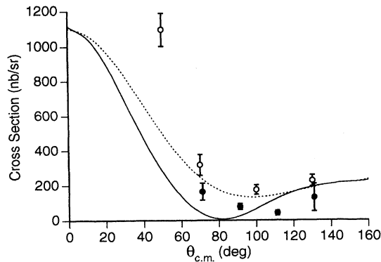
FIG. 2. The ^{15}\text{N} cross section at 170 MeV. Open circles: data of Liesefeld et al. [13]. Solid circles: data of Kobayashi et al. [14]. Solid curve: calculation of Bennhold et al. [15] using (0 + 2h\omega) wave functions. Dashed curve: calculation using 1p -shell only wave functions.
