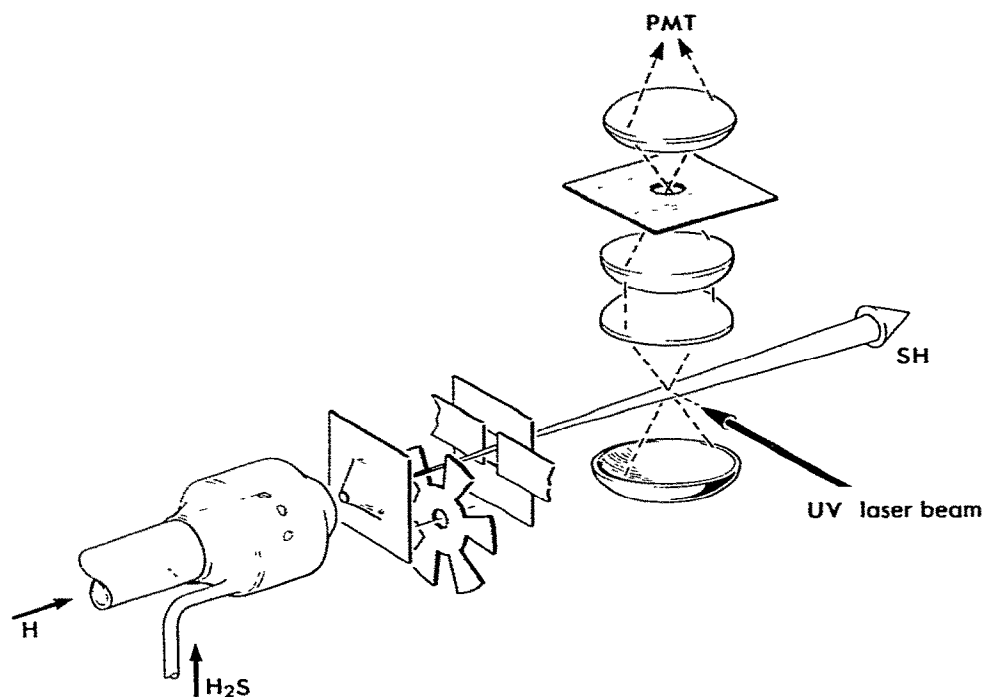
Fig. 1. View of the laser-molecular-beam spectrometer.
