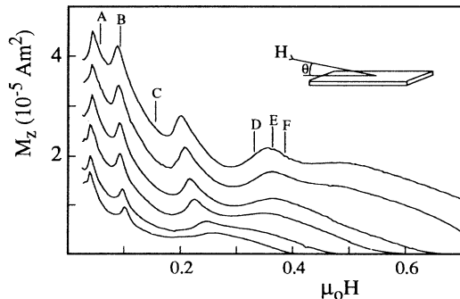
FIG. 1. Field dependence of the magnetic moment M_z measured with the applied field H at \theta = 1^\circ . The curves were obtained at temperatures T = 1.8 , T = 2.3 , T = 2.7 , T = 3.2 , T = 3.7 , and T = 4.1 K (from top to bottom). The letters A-F refer to the vortex distributions shown in Fig. 3.
