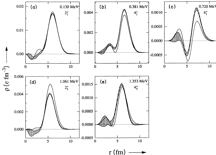
FIG. 1. Transition densities of the ground-state band and the \gamma band of ^{150}\text{Nd} as obtained from experiment (curves with error band) are compared to results of microscopic calculations (solid line). The (a) 2_1^+ state, the (b) 4_1^+ state, the (c) 6_1^+ state, the (d) 2_3^+ state, and the (e) 4_3^+ state are shown. The error bands include the statistical errors as well as the model or incompleteness error.
