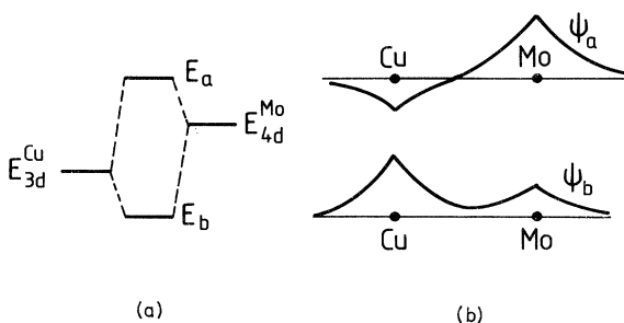
FIG. 3. (a) Schematic representation of the hybridization of the atomic Cu and Mo levels into bonding and antibonding energy levels E_b, E_a . (b) Schematic form of the bonding and antibonding wave functions at the Cu and Mo sites.
