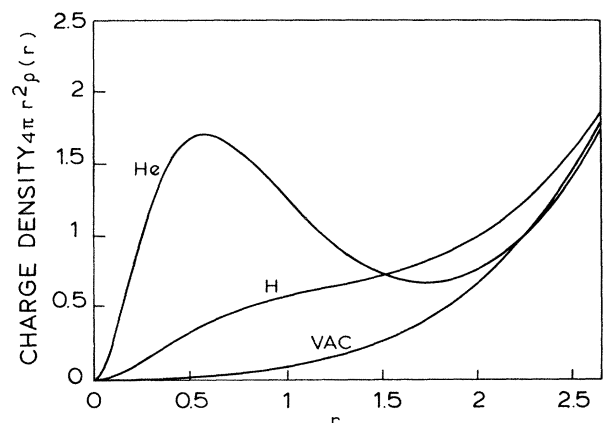
FIG. 12. Spherically averaged charge density (a.u.) in the Wigner-Seitz cell of the vacancy and of substitutional H and He.
