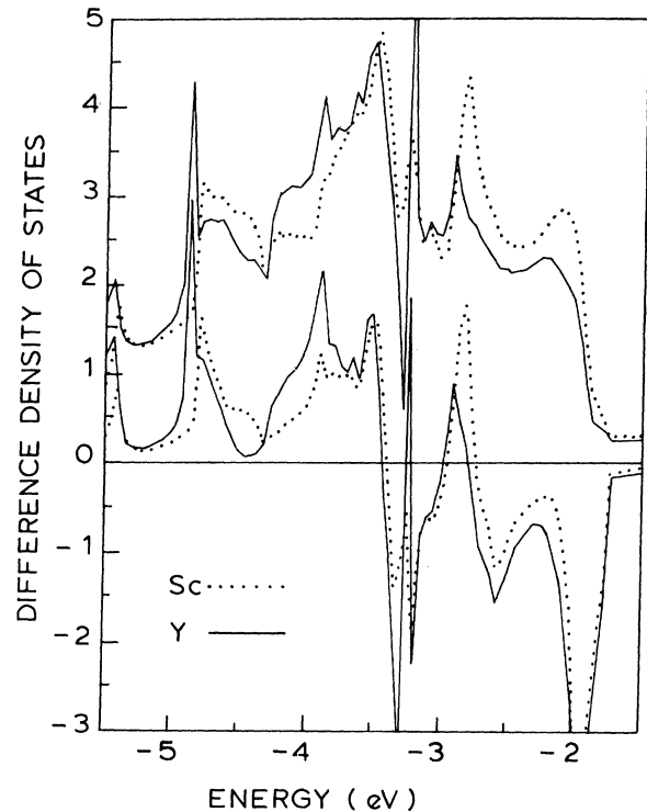
FIG. 7. LDOS (upper curves) and difference LDOS (lower curves) in the Cu-neighbor Wigner-Seitz cell of elements at the beginning of the 3d and 4d series.
