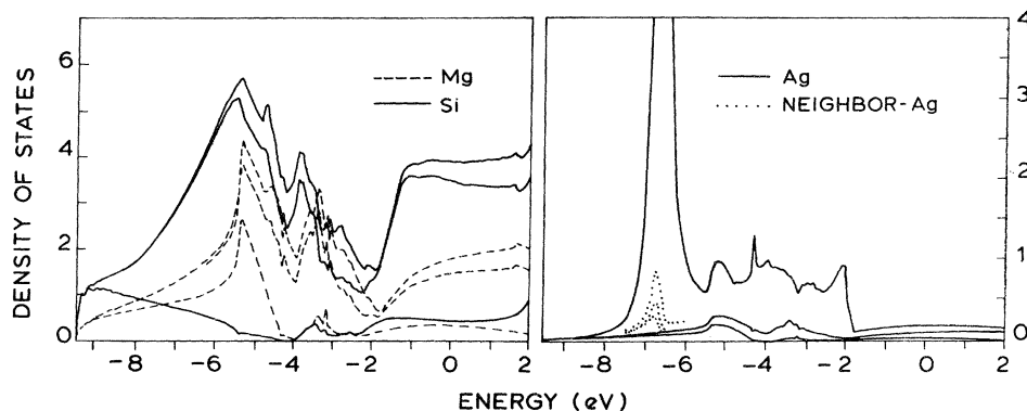
FIG. 13. LDOS in the impurity Wigner-Seitz cell of Mg, Si, and Ag. The influence of the Ag virtual bound state on the LDOS of a Cu neighbor is also shown (dotted).
