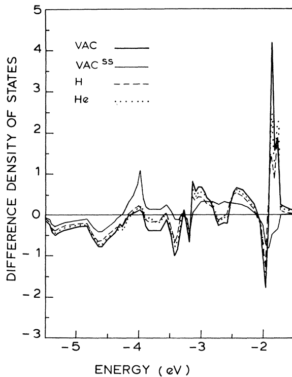
FIG. 11. Difference LDOS in the Cu-neighbor cell of the vacancy and of substitutional H and He.
