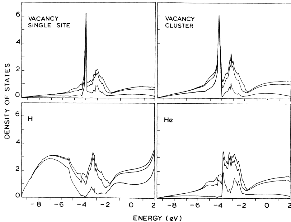
FIG. 10. LDOS of the vacancy and of substitutional H and He impurities. The bound state of He is not shown. For the vacancy both the single-site result and the present "cluster" result are given.
