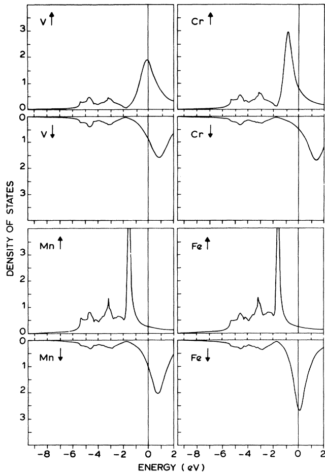
FIG. 8. LDOS in the impurity Wigner-Seitz cell for majority ( \uparrow ) and minority ( \downarrow ) spin of some 3d impurities in Cu.
