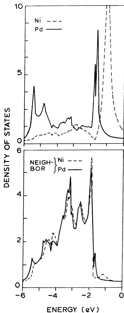
FIG. 6. LDOS in the impurity Wigner-Seitz cell and Cu-neighbor Wigner-Seitz cell of elements from the end of the 3d and 4d series.
