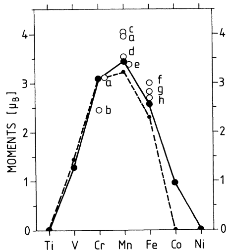
FIG. 9. Local moments in the impurity Wigner-Seitz cell for 3d impurities in Cu. ●, present calculations; •, SSC; ○, experimental values. a , W. D. Weiss, Z. Metallk. 58 , 909 (1967); b , M. Vochten, M. Labro, and S. Vynckier, Physica 86-88B , 467 (1977); c , C. M. Hurd, J. Phys. Chem. Solids 30 , 539 (1969); d , J. R. Davies and T. J. Hicks, J. Phys. F 9 , 753 (1979); e , Ref. 56; f , J. R. Davies and T. J. Hicks, J. Phys. F 9 , L7 (1979); g , P. Steiner, S. Hüfner, and W. V. Zdrojewsky, Phys. Rev. B 10 , 4704 (1974).
