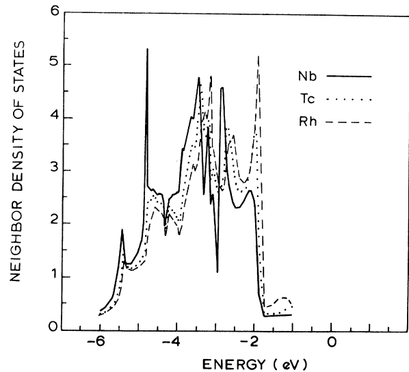
FIG. 4. LDOS in Cu-neighbor Wigner-Seitz cell of some elements from the 4d series. Only the behavior in the Cu d -band energy region and somewhat above it is shown.
