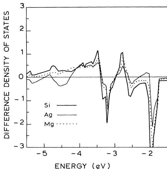
FIG. 14. Difference LDOS in the Cu neighbor Wigner-Seitz cell of Mg, Si, and Ag.
