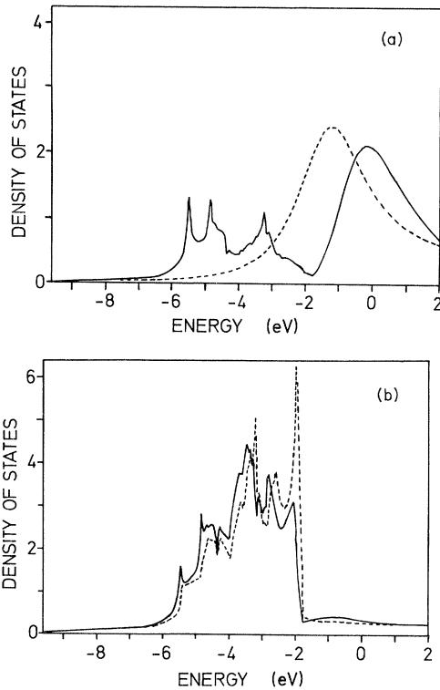
FIG. 2. (a) LDOS for Mo in Cu (solid line). The dotted curve refers to the solution for the single Mo muffin-tin potential in the constant muffin-tin zero-background potential (no "back-scattering"). (b) LDOS of a Cu atom neighboring Mo (solid line) and the unperturbed host density of states of Cu (dotted line).
