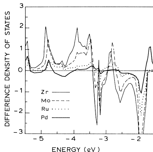
FIG. 5. Difference LDOS in Cu-neighbor Wigner-Seitz cell of some elements from the 4d series.
