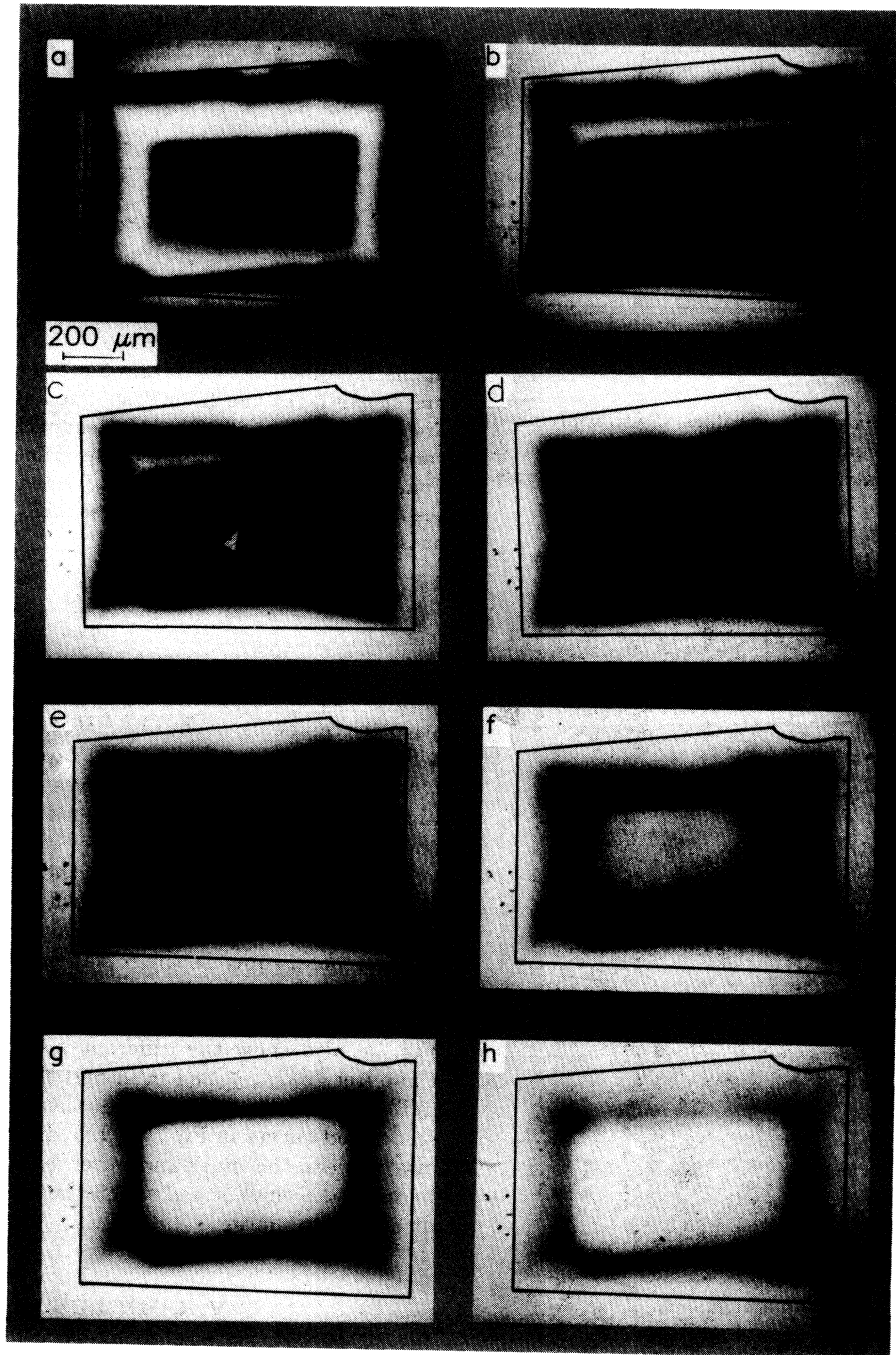
FIG. 23. Flux distribution of the edge-zone-irradiated Bi2212 single crystal when applying a reversed field H_a to the remanent state. (a) \mu_0 H_a = -21 mT, (b) \mu_0 H_a = -85 mT, (c) \mu_0 H_a = -100 mT; here negative flux has started to penetrate the unirradiated zone (white arrow). (d) \mu_0 H_a = -128 mT, (e) \mu_0 H_a = -149 mT, (f) \mu_0 H_a = -171 mT, (g) \mu_0 H_a = -213 mT, (h) \mu_0 H_a = -277 mT.
