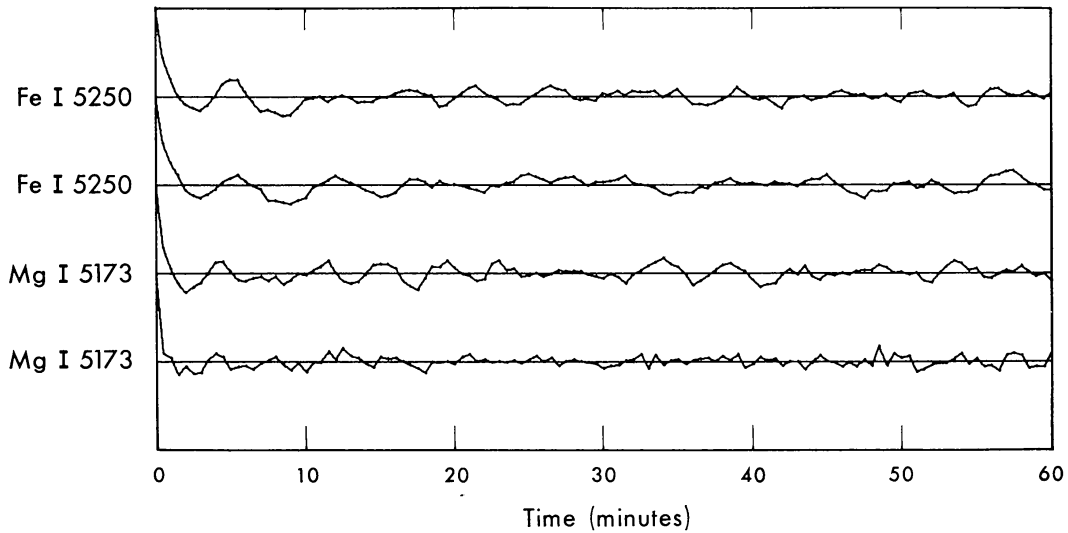
Fig. 2. Autocorrelation of magnetic field for four separate observations. The horizontal line passing through each curve represents a correlation of 0.0. The lines above and below represent +1.0 and -1.0 respectively.
