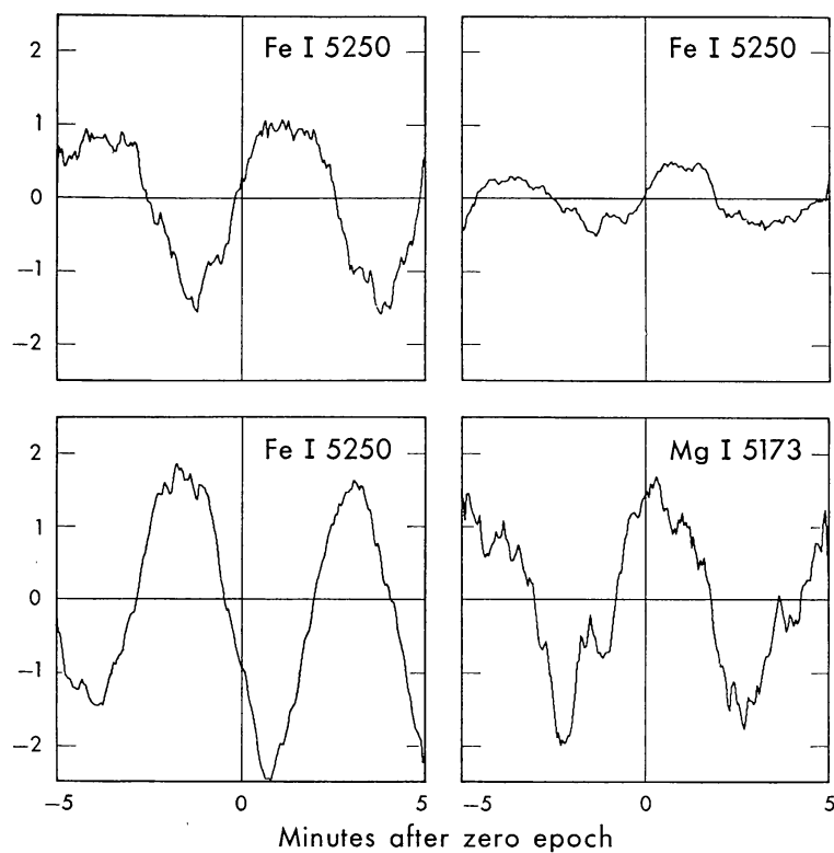
Fig. 6. Four examples of mean magnetic field oscillation profiles during a velocity oscillation as deduced from superposed epoch analysis.
