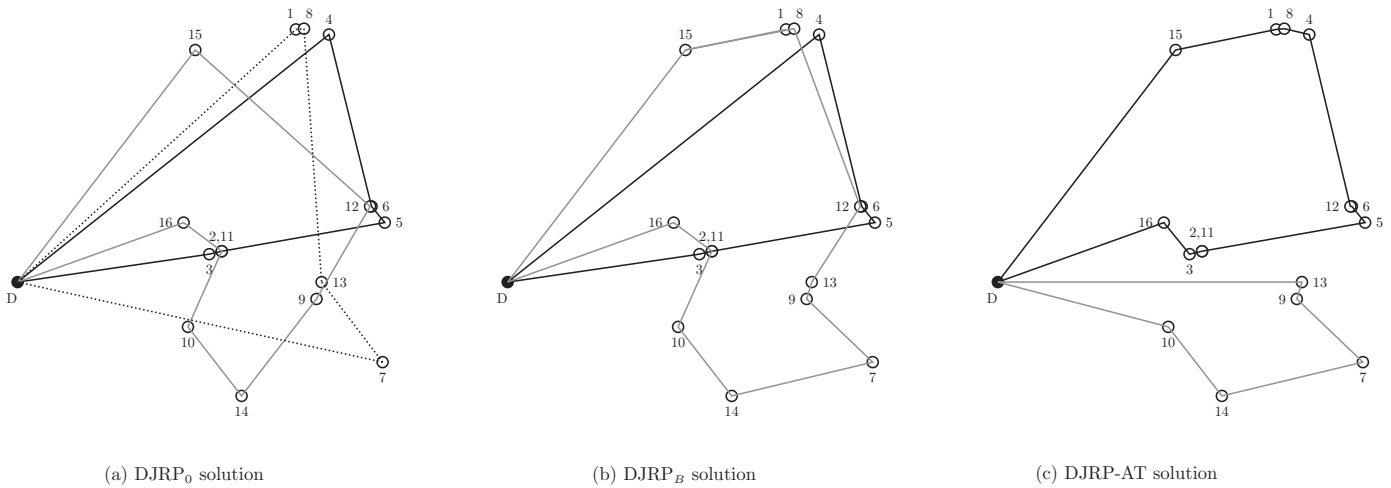
Fig. 3. Inventory based replenishment, DJRP B and DJRP-AT solutions for Region 1 ( k M = 11, m = 100, h = 0.2, black route in period 1, gray route in period 2, dotted route in period 3).
